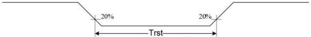
Figure 13.5: Reset timing
