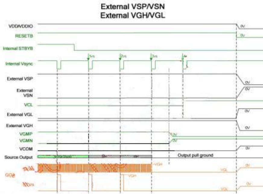
Power off sequence with PMODE=H
