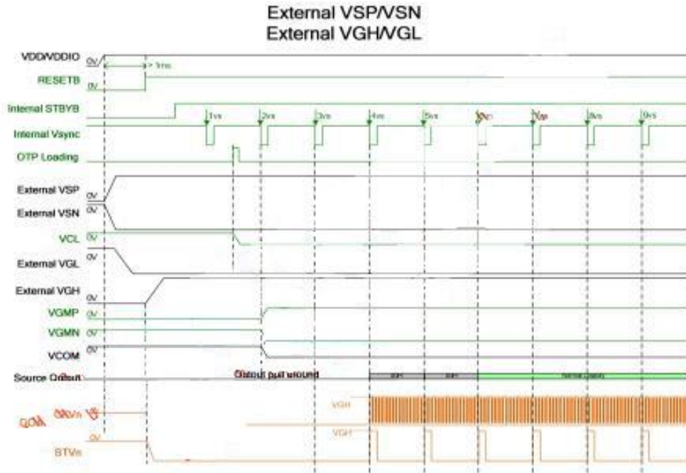
Power on sequence with PMODE=H
